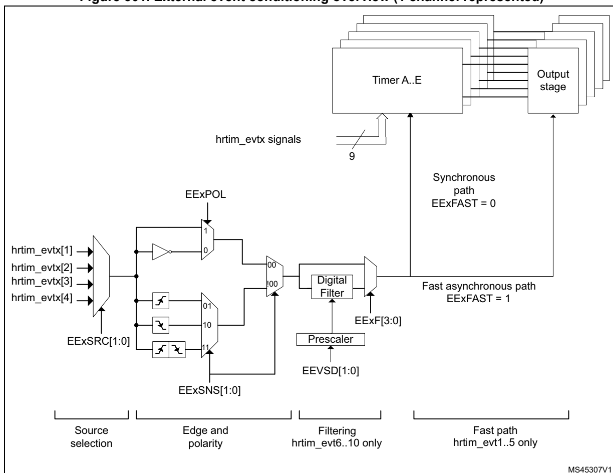
Figure 301. External event conditioning overview (1 channel represented)
