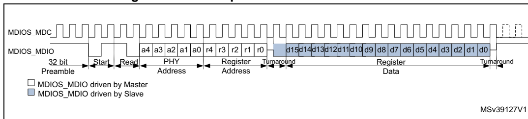
Figure 695. MDIO protocol read frame waveform
