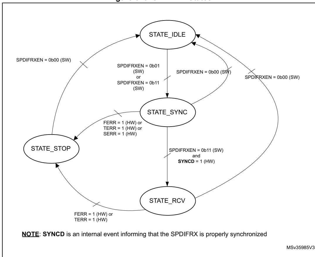
Figure 675. SPDIFRX States
