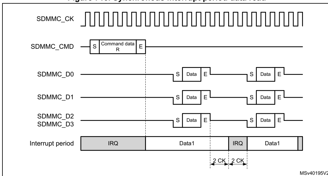
Figure 713. Synchronous interrupt period data read
