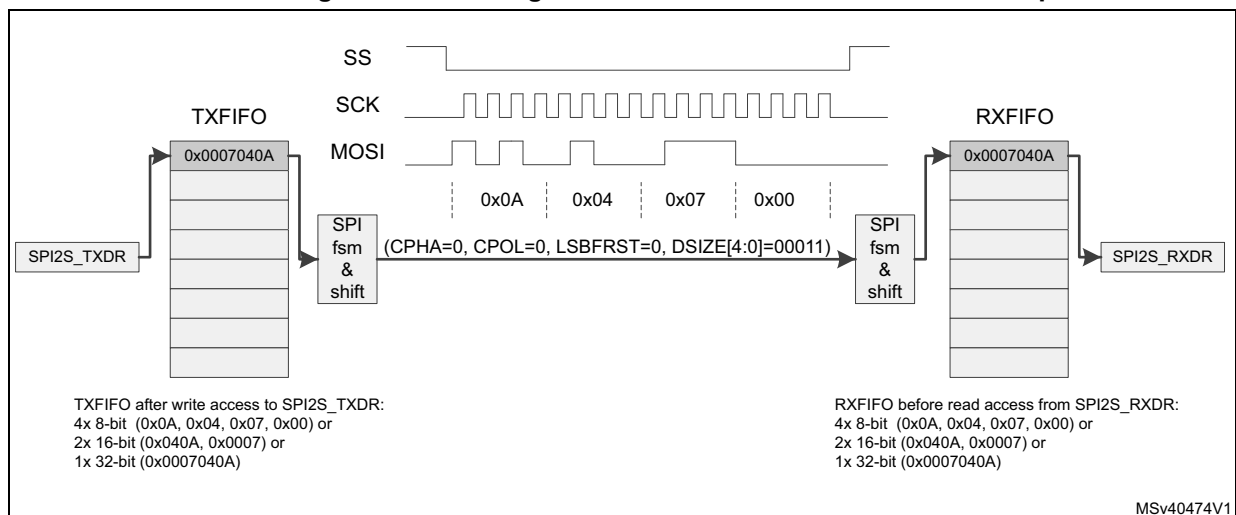
Figure 621. Packing data in FIFO for transmission and reception
