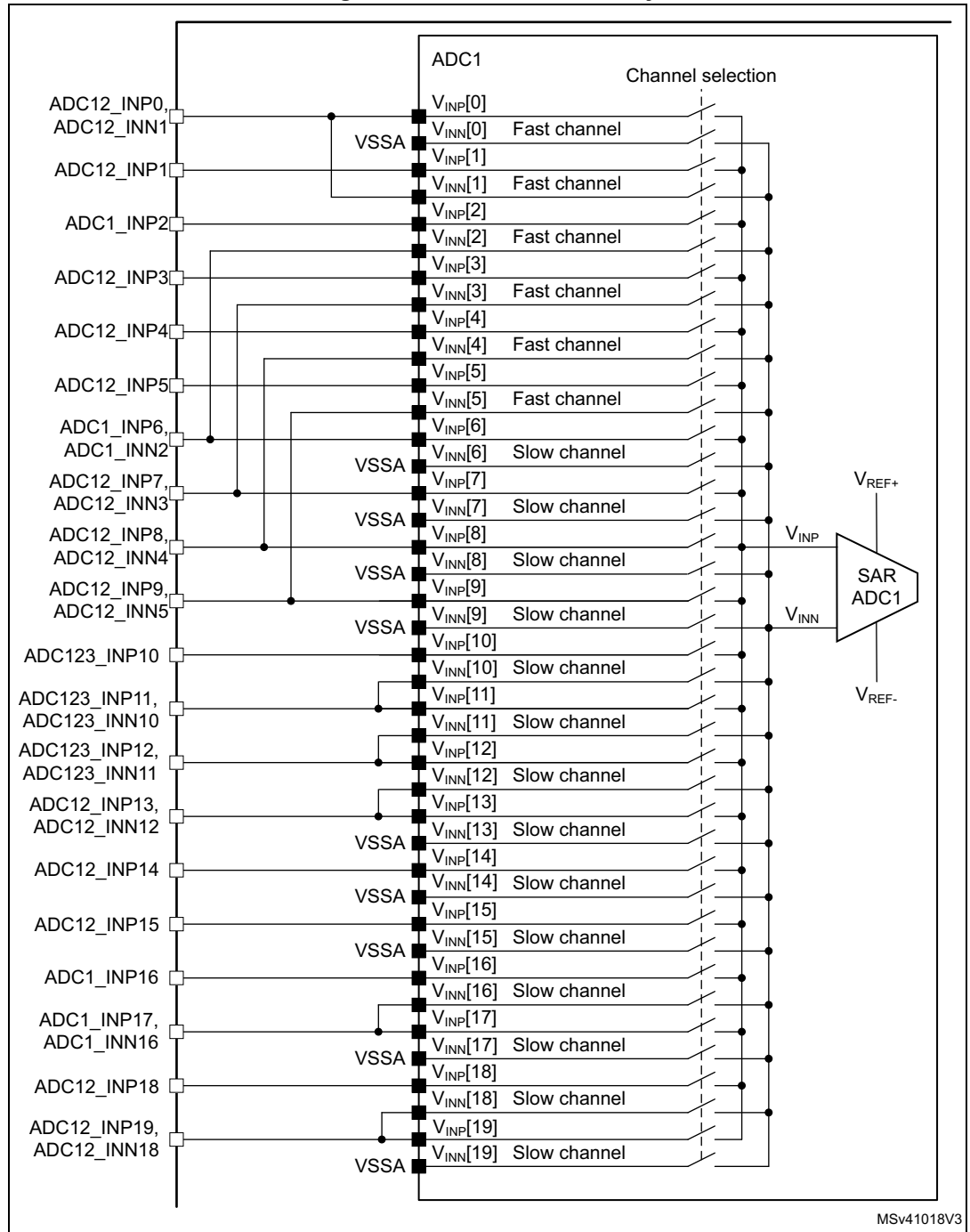
Figure 138. ADC1 connectivity
