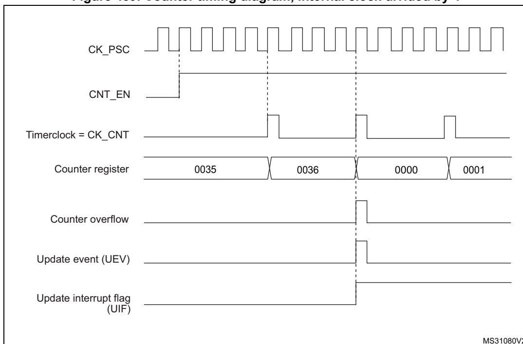
Figure 459. Counter timing diagram, internal clock divided by 4
