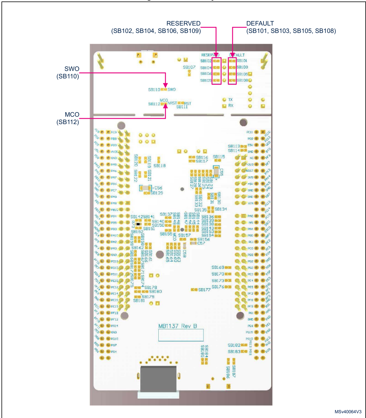
Figure 5. Bottom layout
