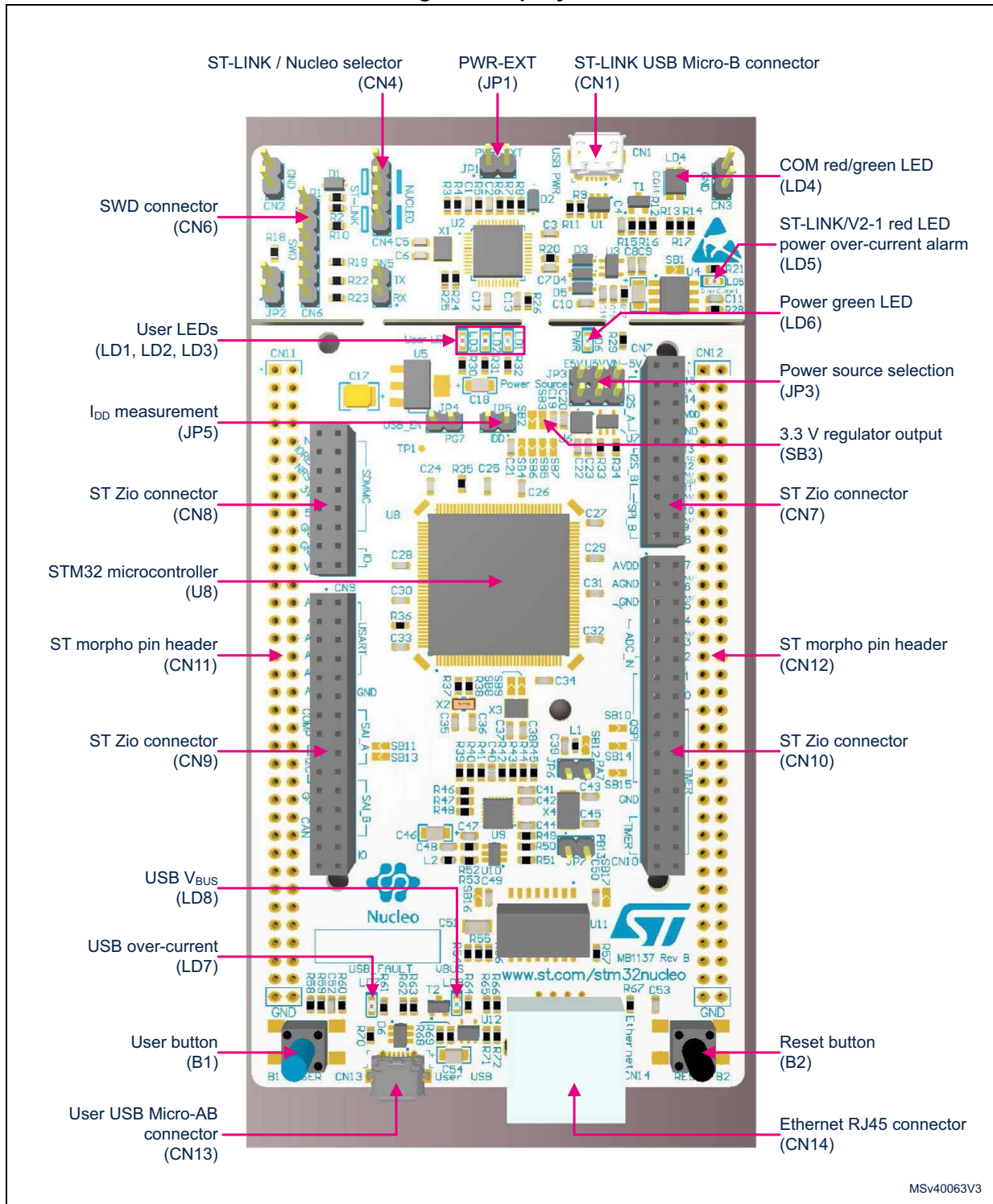
Figure 4. Top layout
