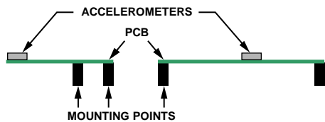
Figure 35. Incorrectly Placed Accelerometers
